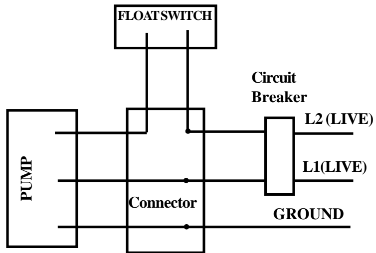
Direct Wiring
