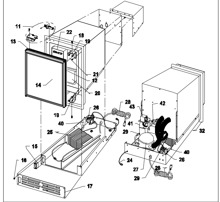
Exploded view of Item #21
