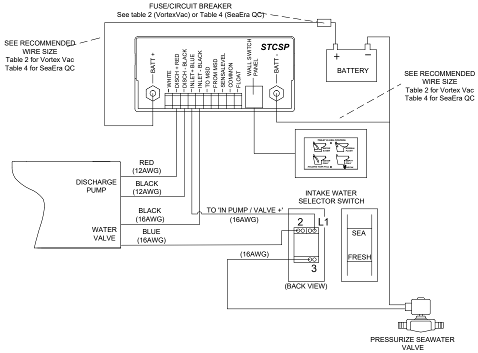
FIG 5 WIRING FOR SMART TOILET CONTROL SEA/FRESH MODEL: PRESSURIZED SEAWATER VALVE
