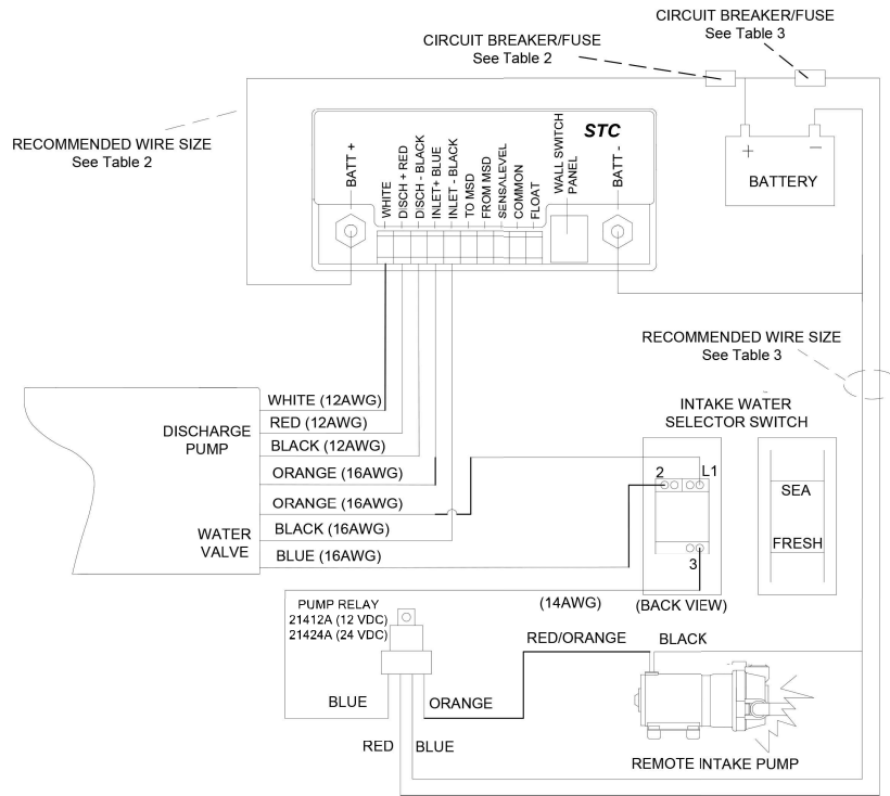
FIG 5 WIRING FOR FLUSH HANDLE WITH SMART TOILET CONTROL SEA/FRESH 03 MODELS
